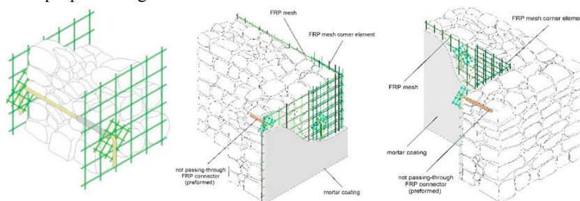
Fig. 2. Fibre Net retrofit intervention system.
