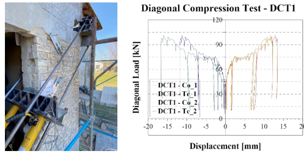
Fig. 3. Diagonal compression test setup and load – diagonal displacement diagrams.
