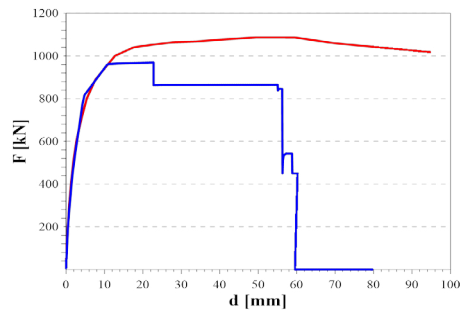
Fig. 7. Experimental (red) and numerical (blue) force-displacement response curve for building 2.
