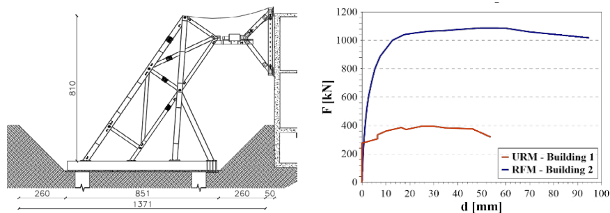
Fig. 6. Scheme of the push structure and experimental push-over diagram.
