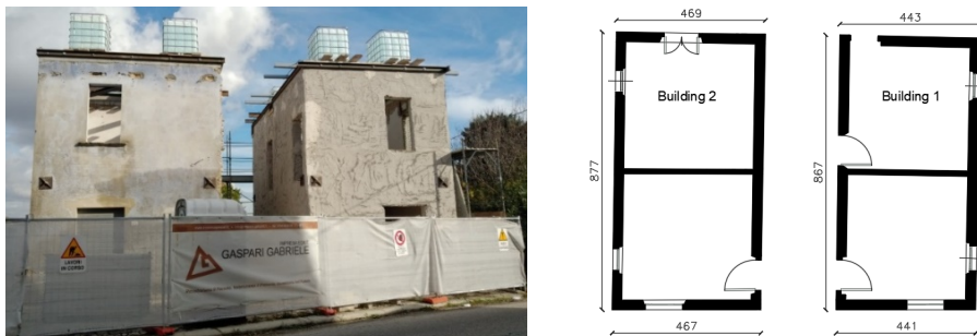
Fig. 2. Building 1 (not consolidated, on the left) and building 2. Plans of the first floors.
