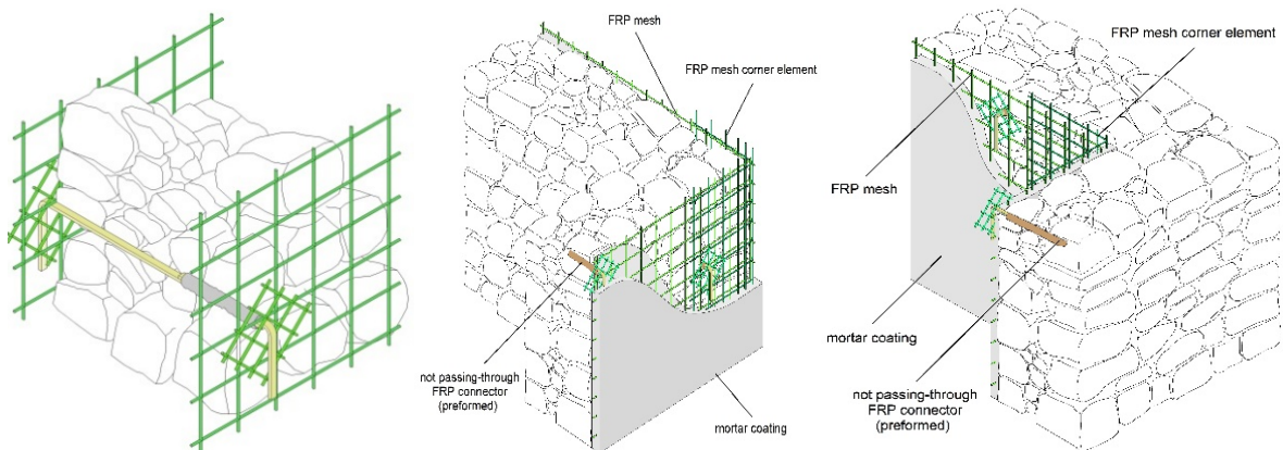
Fig. 4. Fibre Net system.
